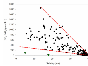
Figure 3. Relationship between \text{NO}_2^- + \text{NO}_3^- concentrations and salinity in surface water at three stations along the Kishon lower estuary between 2002–2021. The bottom green triangles represent measured values at a period of almost no anthropogenic discharge (November 2017) due to a strike at the fertilizer industrial plant. The red lines represent mixing curves between the highest and lowest \text{NO}_2^- + \text{NO}_3^- levels in the fresh/brackish water endmember and the seawater endmember (salinity ~40 psu).
