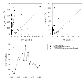
Figure 5. Relationship between \text{NO}_2^- + \text{NO}_3^- (A) or DIN (B) vs. \text{PO}_4^{3-} concentrations in surface water at the Kishon harbor during this study, 2002–2021 (black circle) and measurements performed during 1993–2000 (white triangles, [24,25]). The linear regression slopes for this study and 1993–2000 in panel A are 17.3 and 2.6, and in panel B are 11.3 (or 17.6 excluding the high anomalous value) and 4.6, respectively. The anthropogenic N:P load ratio is shown in panel (C) (grey square, calculated from the source: Israel Ministry of Environmental Protection, 2023 Report on pollutants budget, www.gov.il/bel/departments/guides/kishon_stream_point_pollution_loads/chapter/index-5 ).
