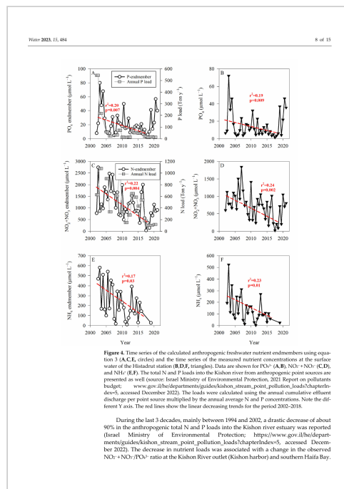
Figure 4. Time series of the calculated anthropogenic freshwater nutrient endmembers (A,C,E, circles) and the time series of the measured nutrient concentrations at the surface water of the Histadrut station (B,D,F, triangles), for PO_4^{3-} , NO_2^- + NO_3^- , and NH_4^+ . The total N and P loads into the Kishon river from anthropogenic point sources are also presented. The red lines show the linear decreasing trends for the period 2002–2018.
