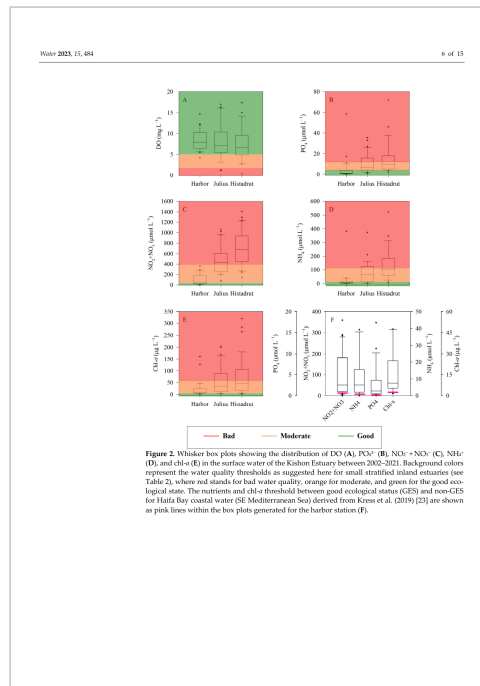
Figure 2. Whisker box plots showing the distribution of DO (A), PO_4^{3-} (B), NO_2^- + NO_3^- (C), NH_4^+ (D), and chl-a (E) in the surface water of the Kishon Estuary between 2002–2021. Background colors represent the water quality thresholds suggested in this study for small stratified inland estuaries (Table 2): red = bad, orange = moderate, green = good ecological state. The nutrient and chl-a thresholds between good ecological status (GES) and non-GES for Haifa Bay coastal water (SE Mediterranean Sea) derived from Kress et al. (2019) [23], are shown as pink lines within the box plots generated for the harbor station (F).
