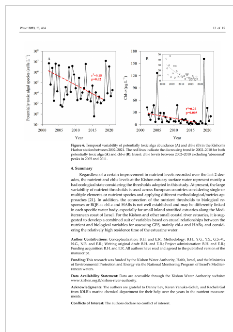
Figure 6. Temporal variability of potentially toxic alga abundance (A) and chl- a (B) in the Kishon's Harbor station between 2002–2021. The red lines indicate the decreasing trend in 2002–2018 for both potentially toxic alga (A) and chl- a (B).
